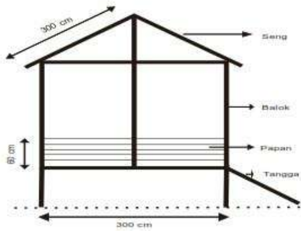
Tampak Samping
