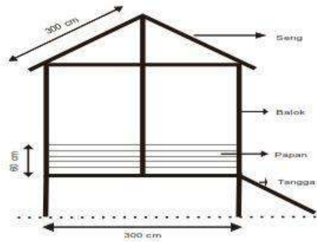
Tampak Samping
